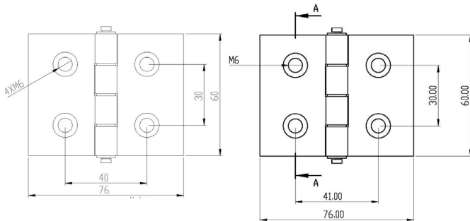
HTA40A / HTA40B
