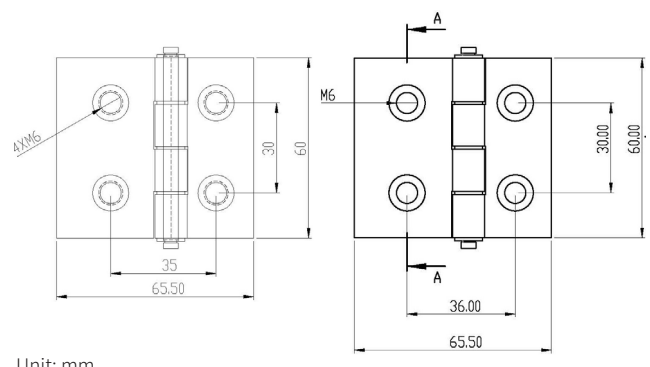
HTA35A / HTA35B
