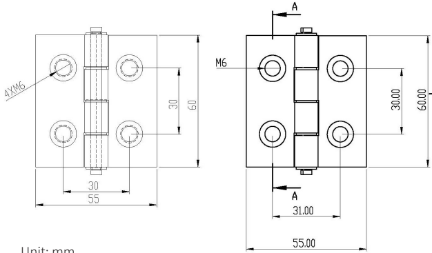
HTA30A / HTA30B
